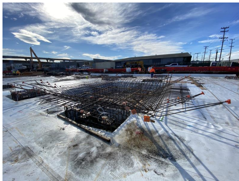
Waterproofing and Rebar at Elevator Pit – December 31, 2019
