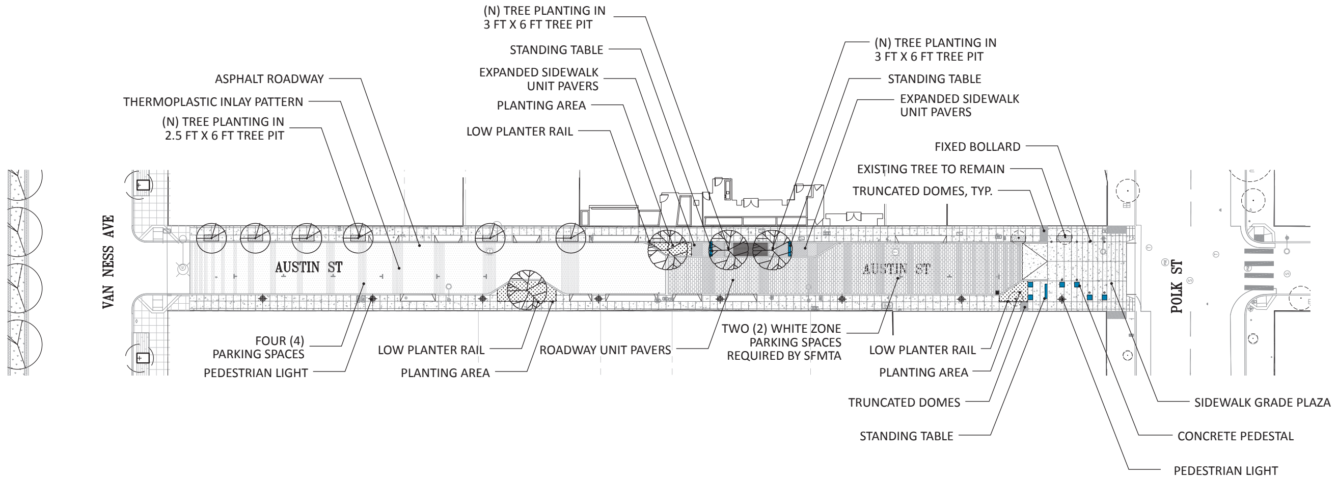
SITE PLAN Austin Alley: Proposed Design Concept Polk Streetscape. January 12, 2018
