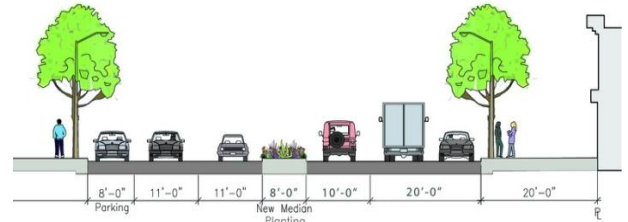
Planned installation of a median and street trees
